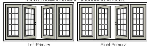
FOUR PANEL SYSTEMS – DOUBLE OPERATOR
