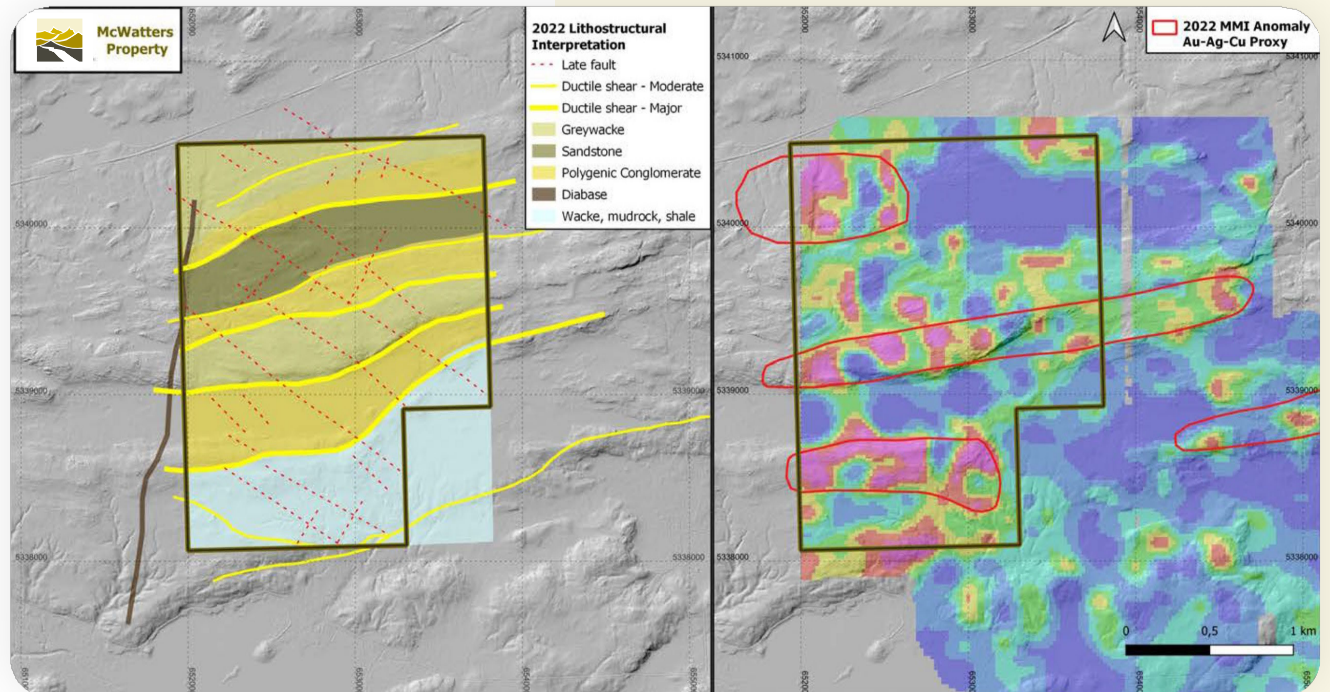
Vertical Gradient of RTP (M-PASS survey 2022)
