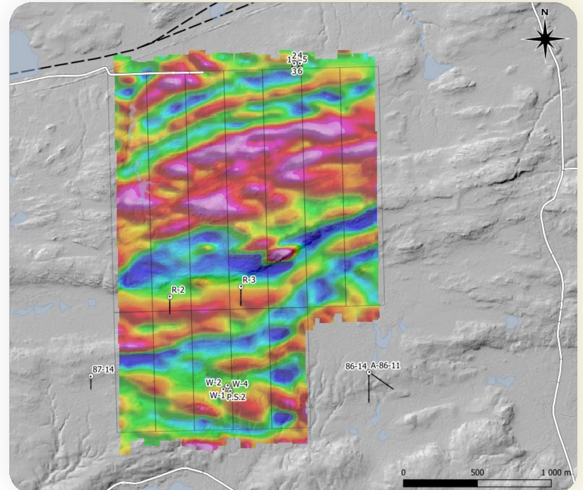
Vertical Gradient of RTP (M-PASS survey 2022)
