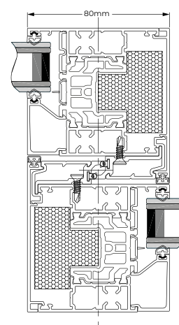
Standard Interlock
