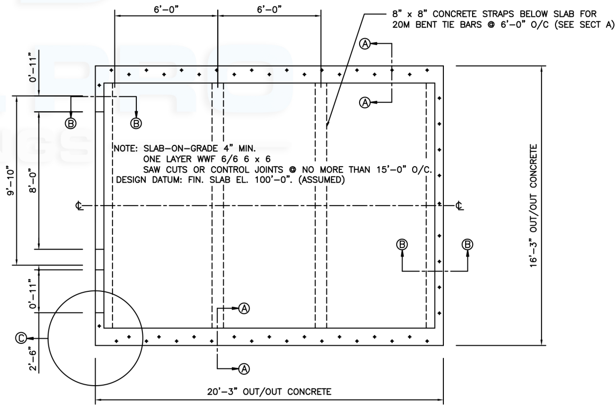
FOUNDATION PLAN
