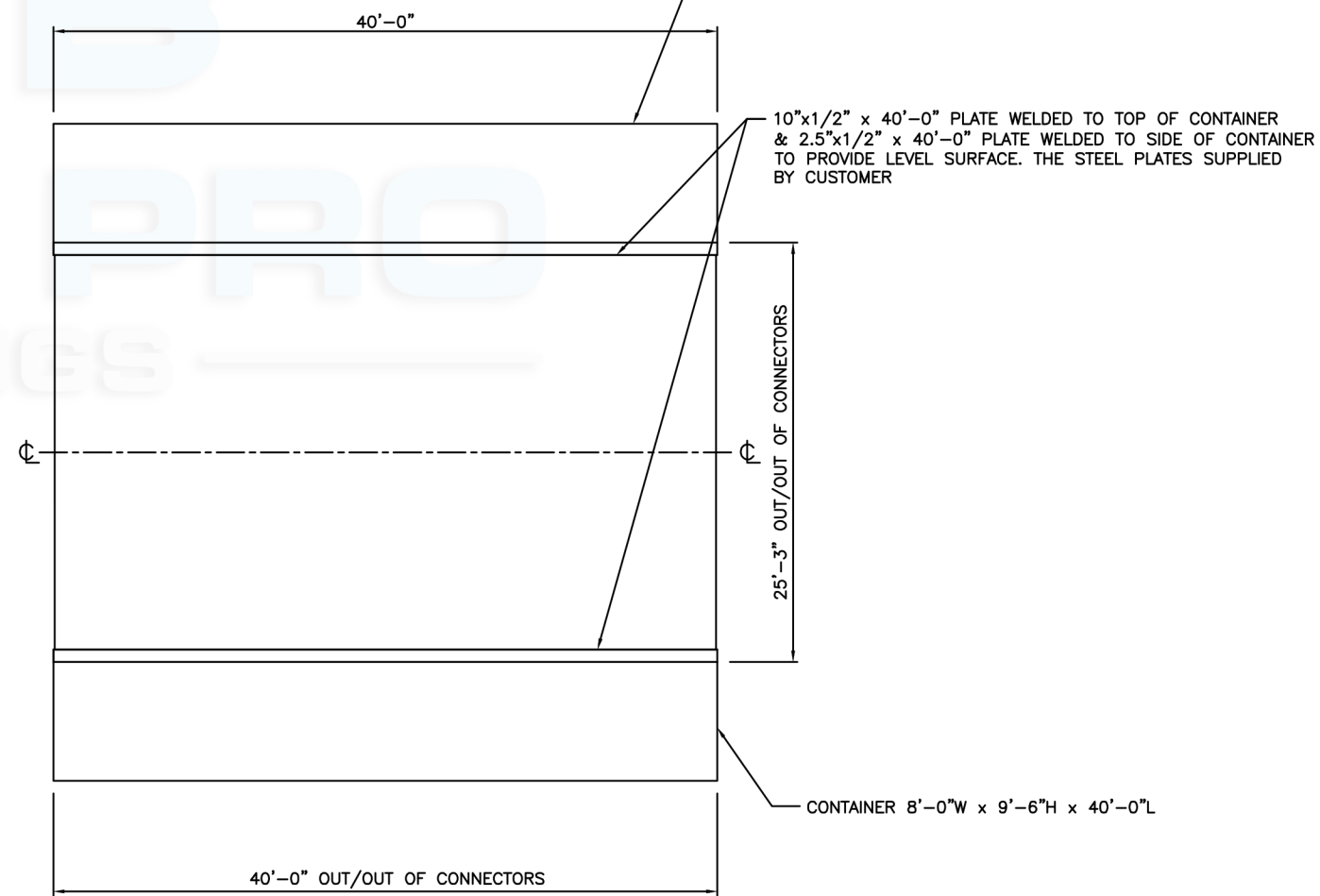
FOUNDATION PLAN
