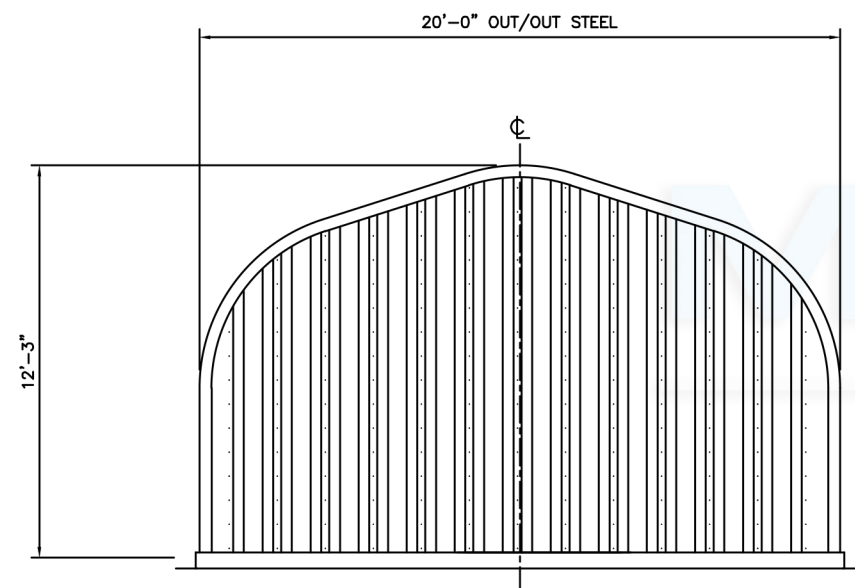
REAR ELEVATION
