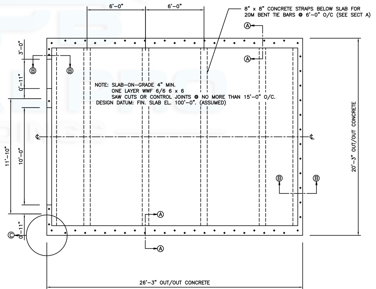
FOUNDATION PLAN
