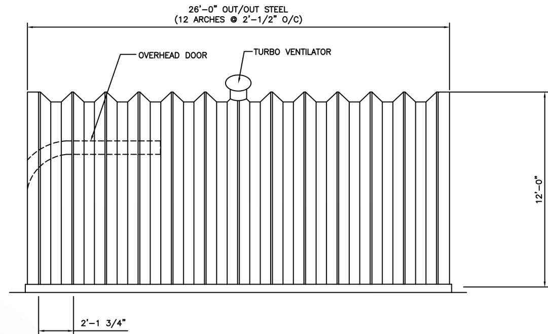
SIDE ELEVATION
