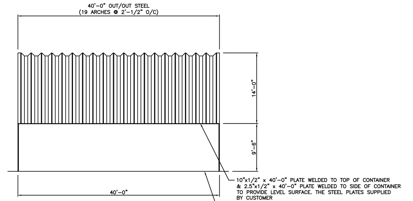
SIDE ELEVATION
