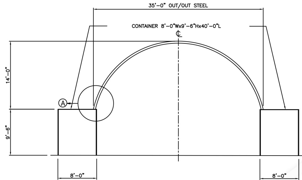
FRONT ELEVATION
