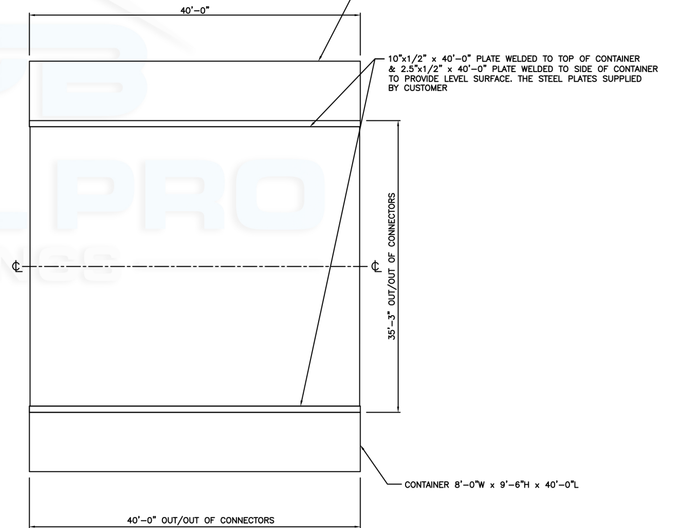
FOUNDATION PLAN
