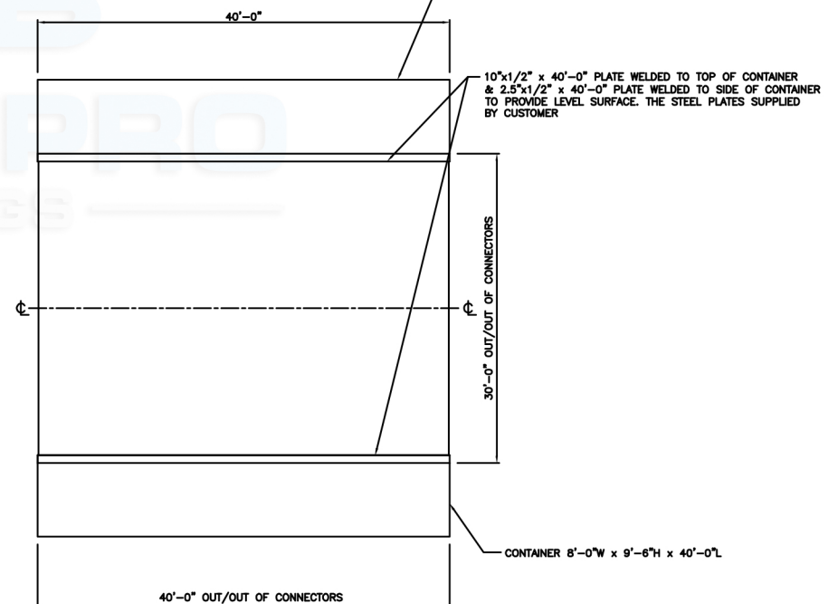
FOUNDATION PLAN
