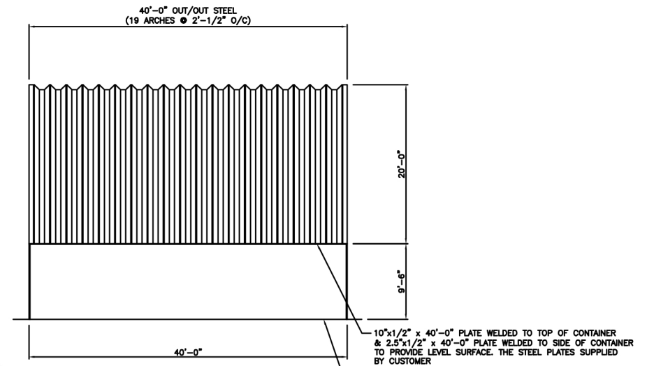
SIDE ELEVATION
