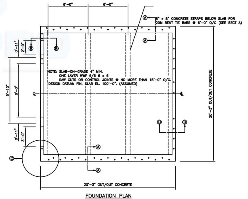
FOUNDATION PLAN
