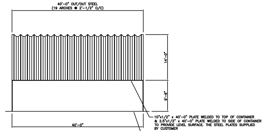
SIDE ELEVATION
