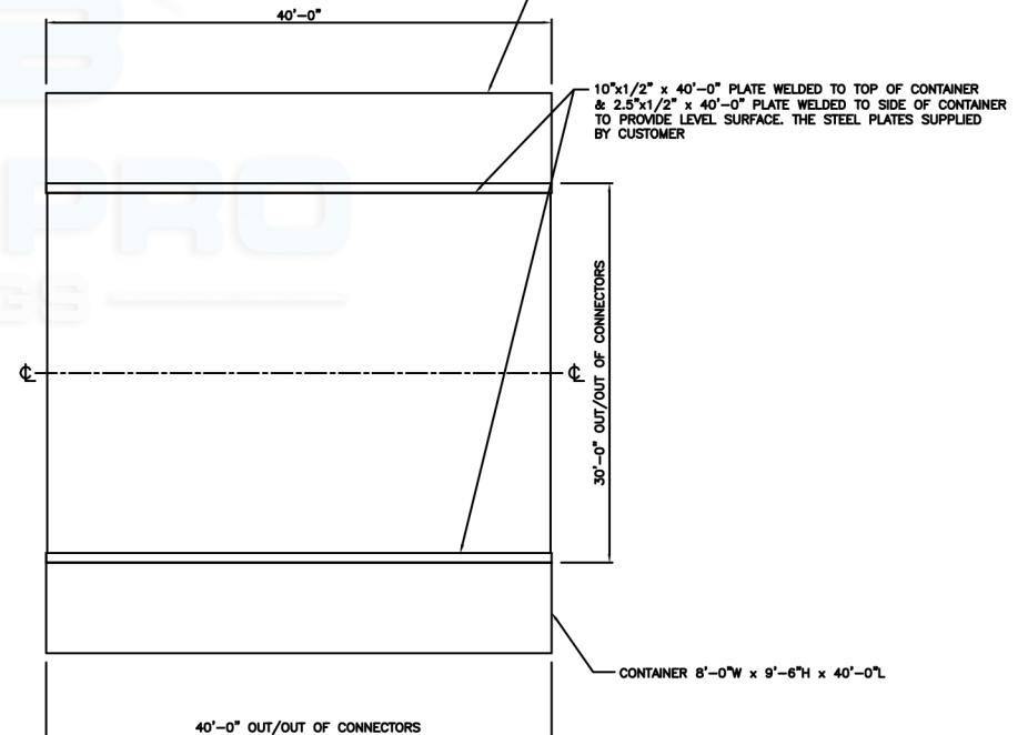
FOUNDATION PLAN
