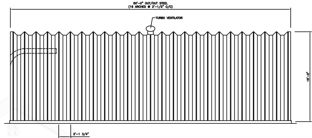
SIDE ELEVATION
