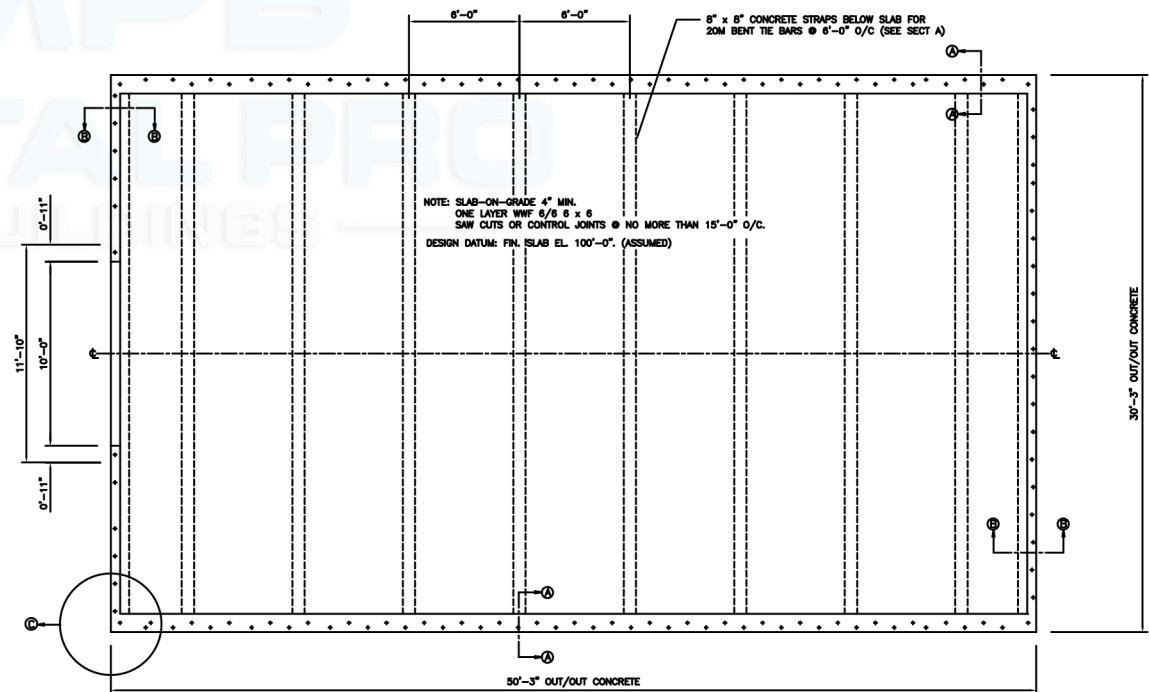
FOUNDATION PLAN
