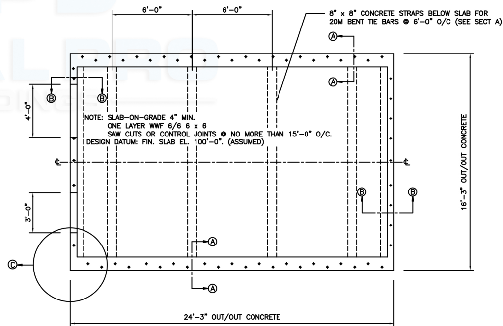
FOUNDATION PLAN
