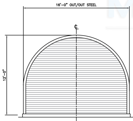
REAR ELEVATION
