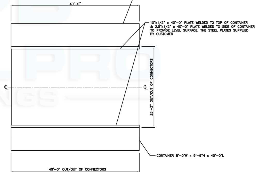
FOUNDATION PLAN
