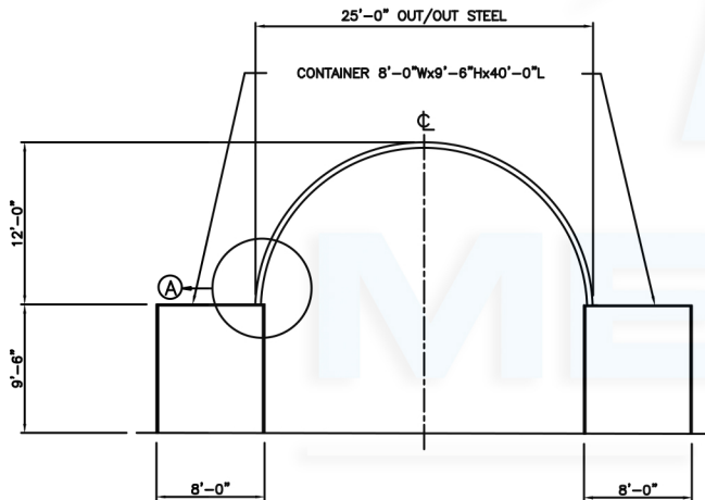
REAR ELEVATION
