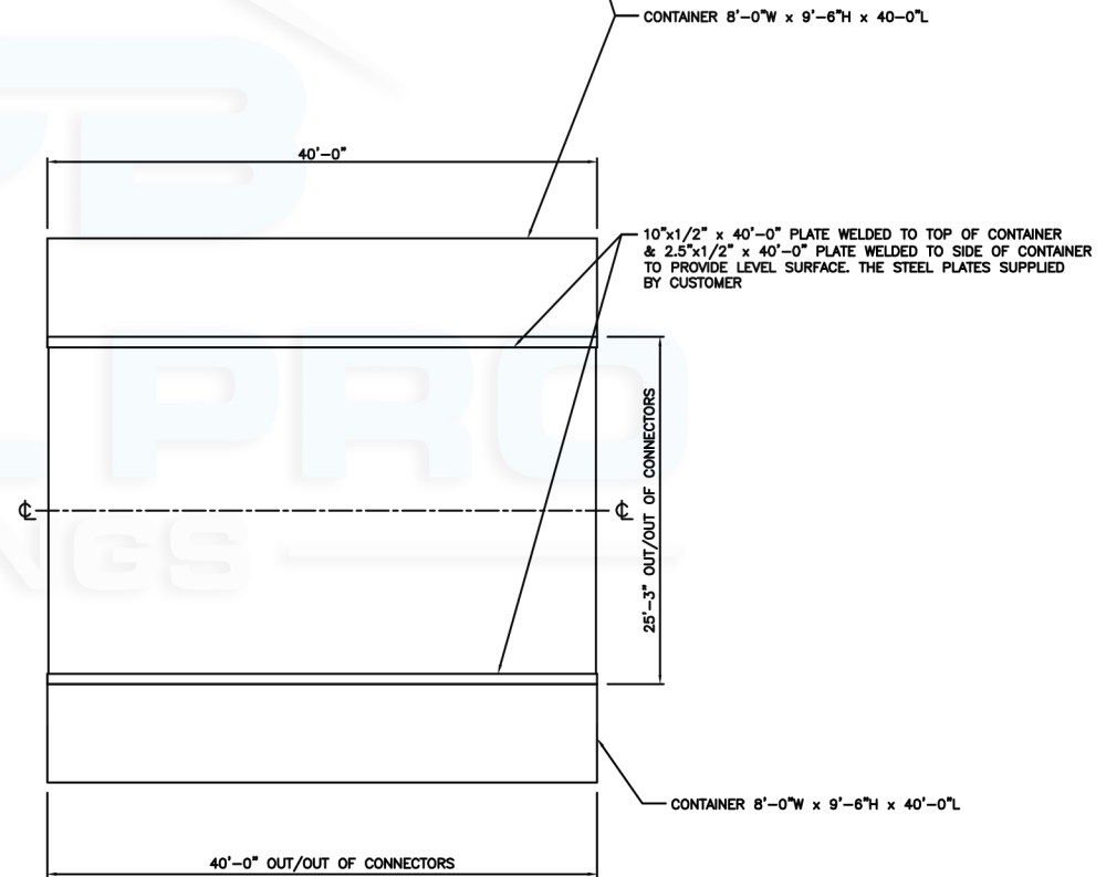
FOUNDATION PLAN
