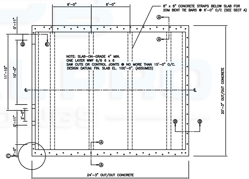
FOUNDATION PLAN
