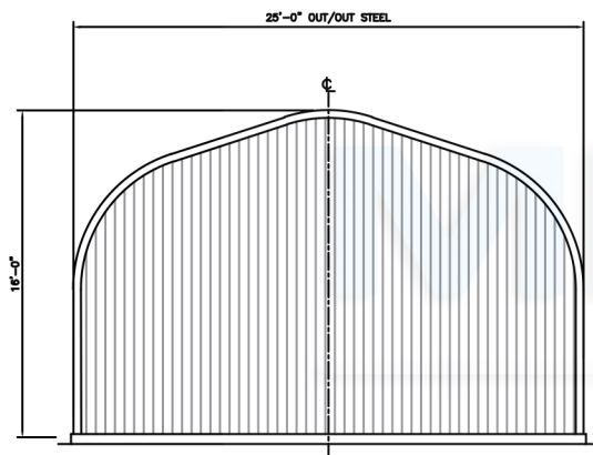
REAR ELEVATION
