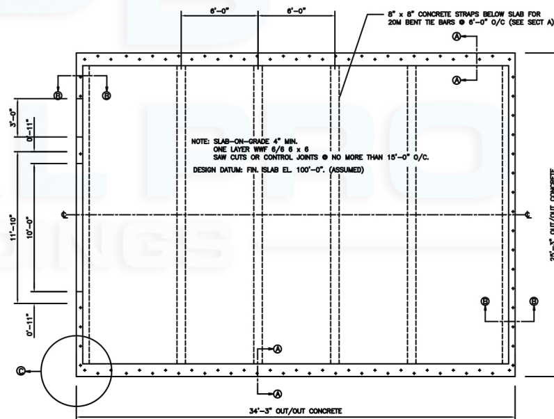
FOUNDATION PLAN
