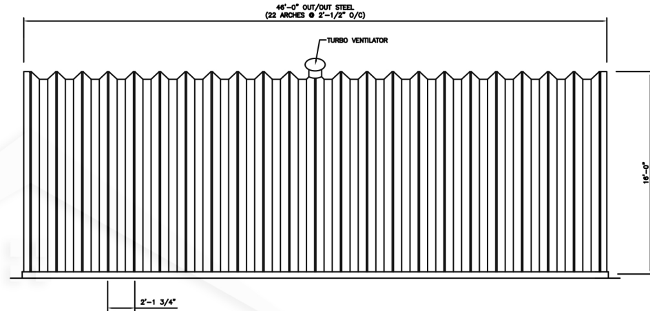
SIDE ELEVATION
