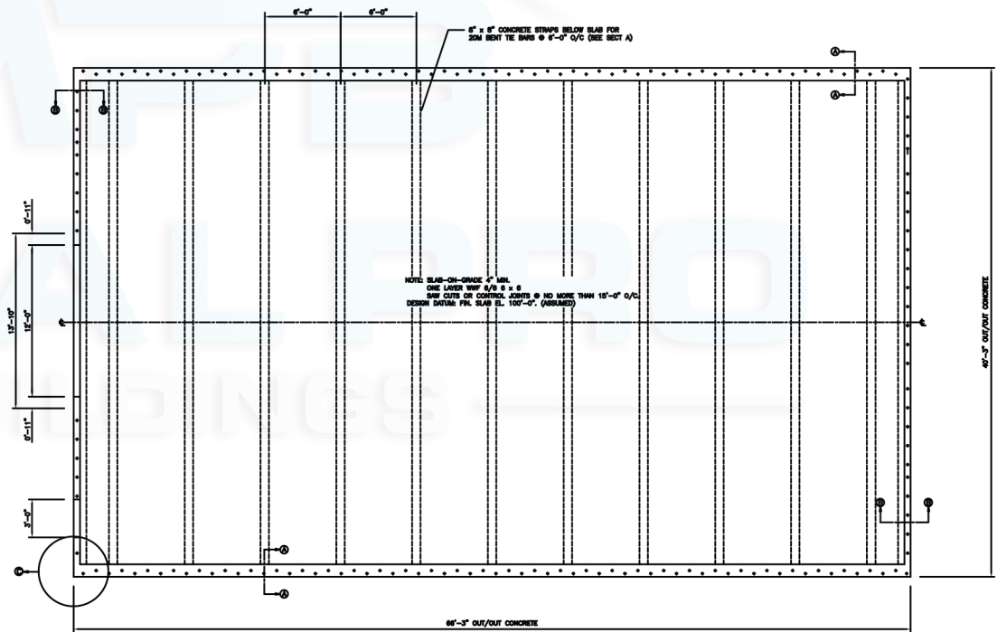
FOUNDATION PLAN
