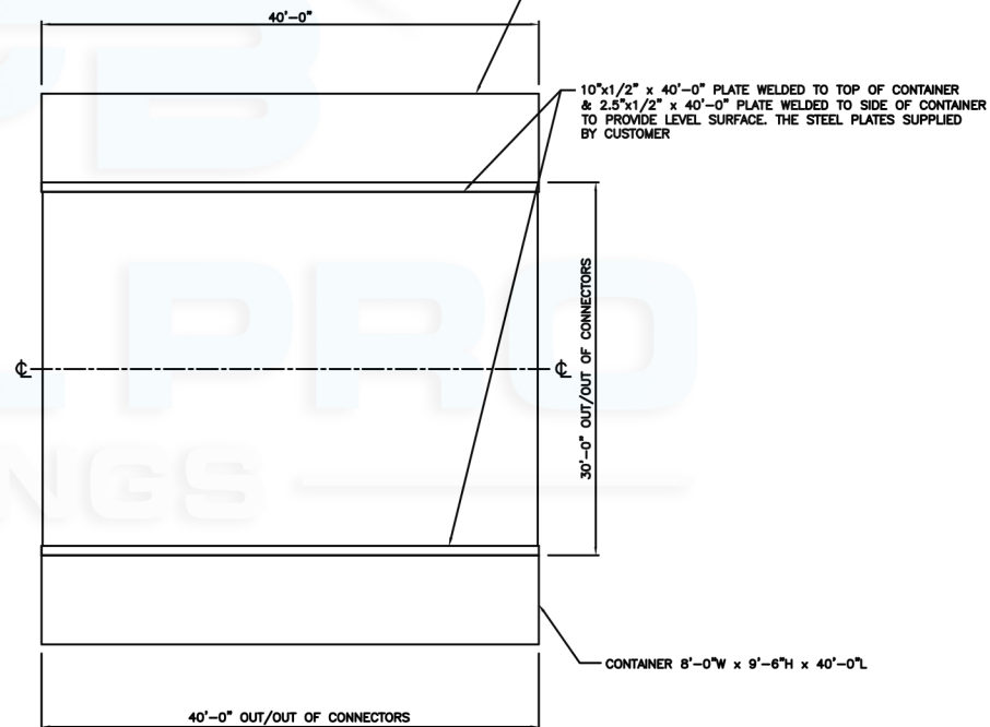
FOUNDATION PLAN
