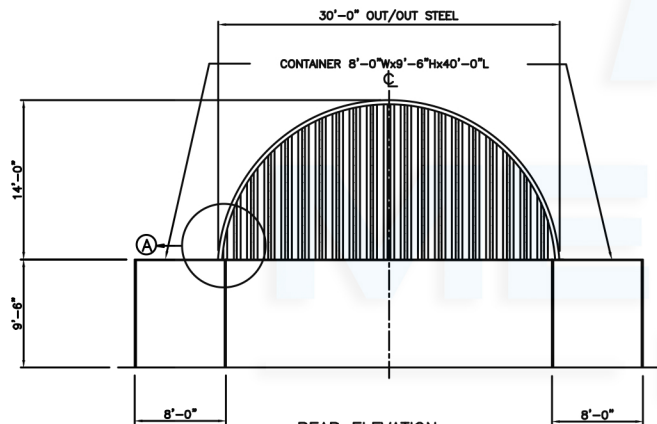
REAR ELEVATION
