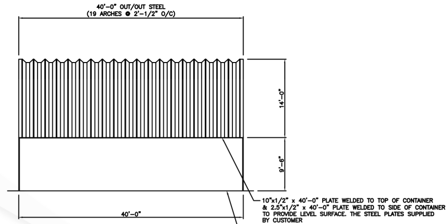
SIDE ELEVATION
