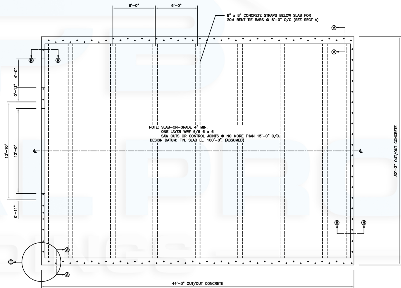
FOUNDATION PLAN
