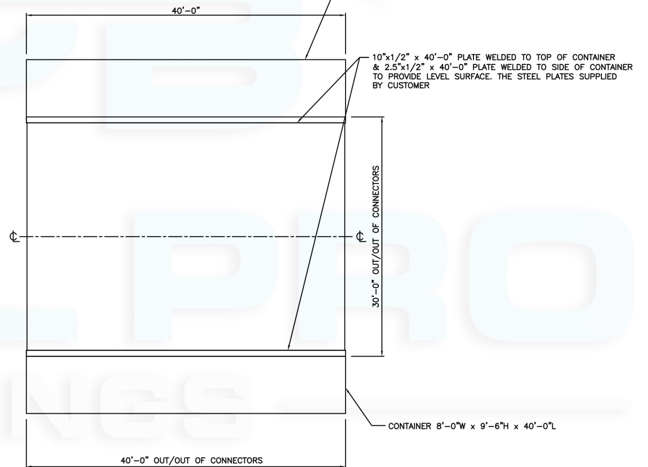
FOUNDATION PLAN
