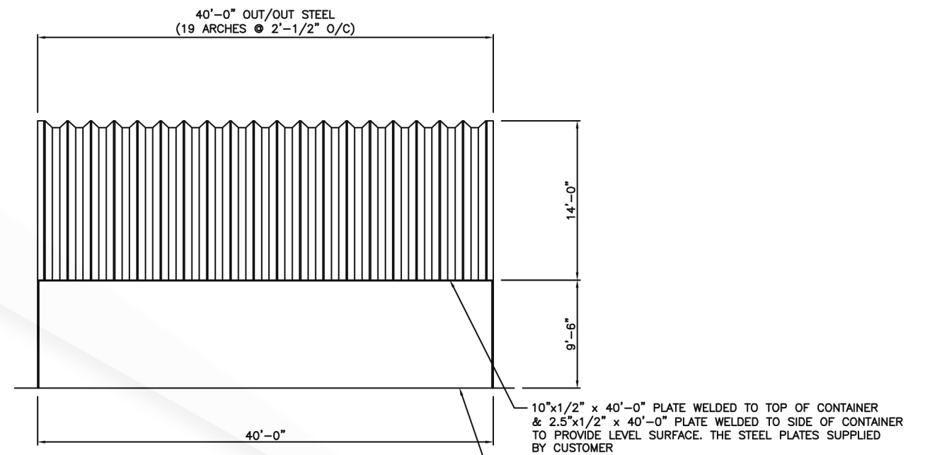
SIDE ELEVATION
