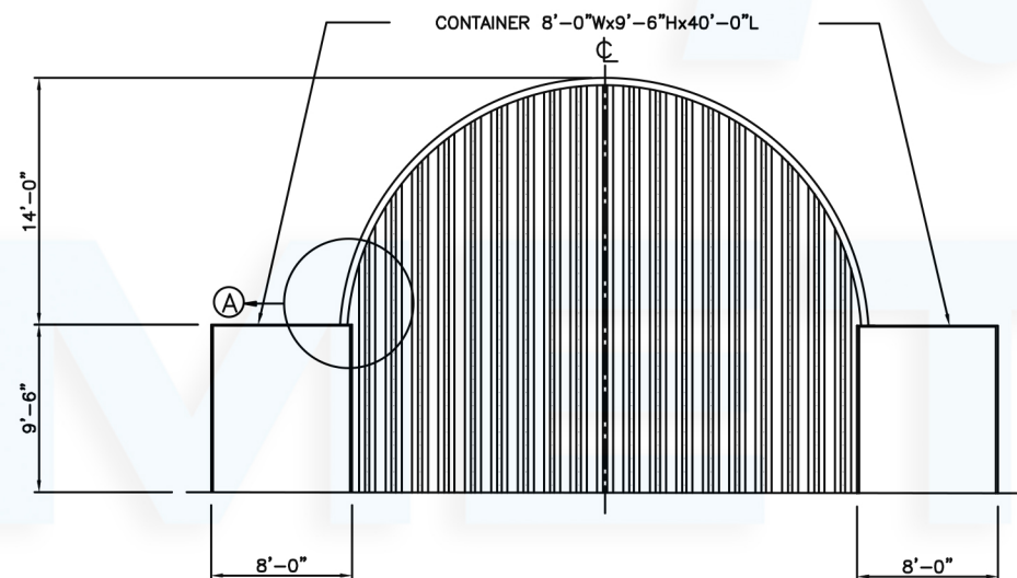
REAR ELEVATION
