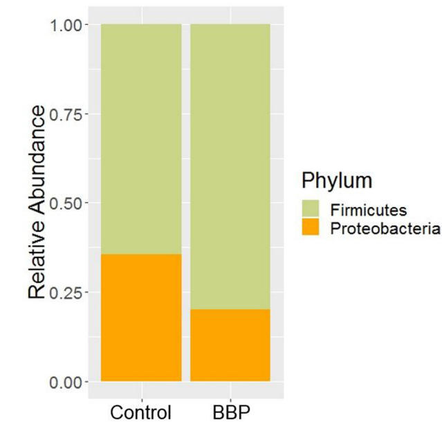
Figure 1. Relative abundance of bacterial phyla recovered from Control and Bacillus base probiotic (BBP) in trial 2.
