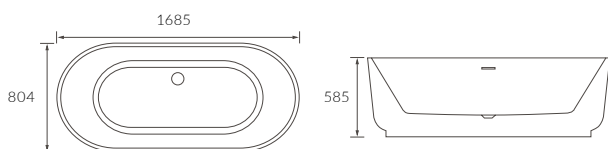
LUGO FLOORSTANDING BATH
