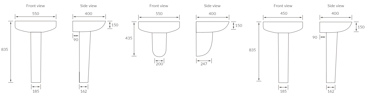
BASIN WITH FULL PEDESTAL 550 x 400mm
