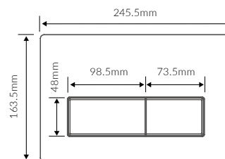
RECTANGLE FLUSH PLATE
