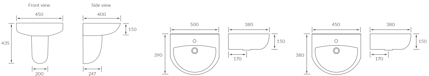
BASIN WITH SEMI PEDESTAL 450 x 400mm
