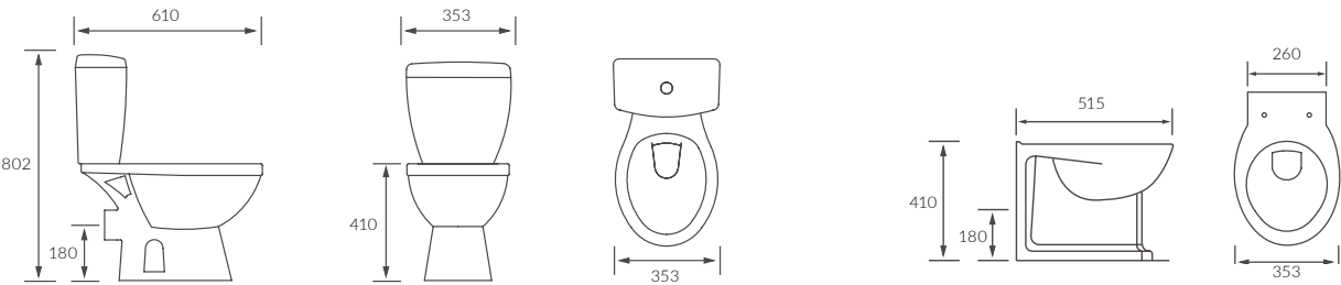
CLOSE COUPLED PAN AND CISTERN Coupling to soil stack: Straight out, straight down, Left or Right Distance from soil pipe spigot to wall: 100mm Cistern inlet position: Left
