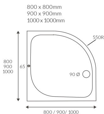
LOW PROFILE QUADRANT TRAYS
