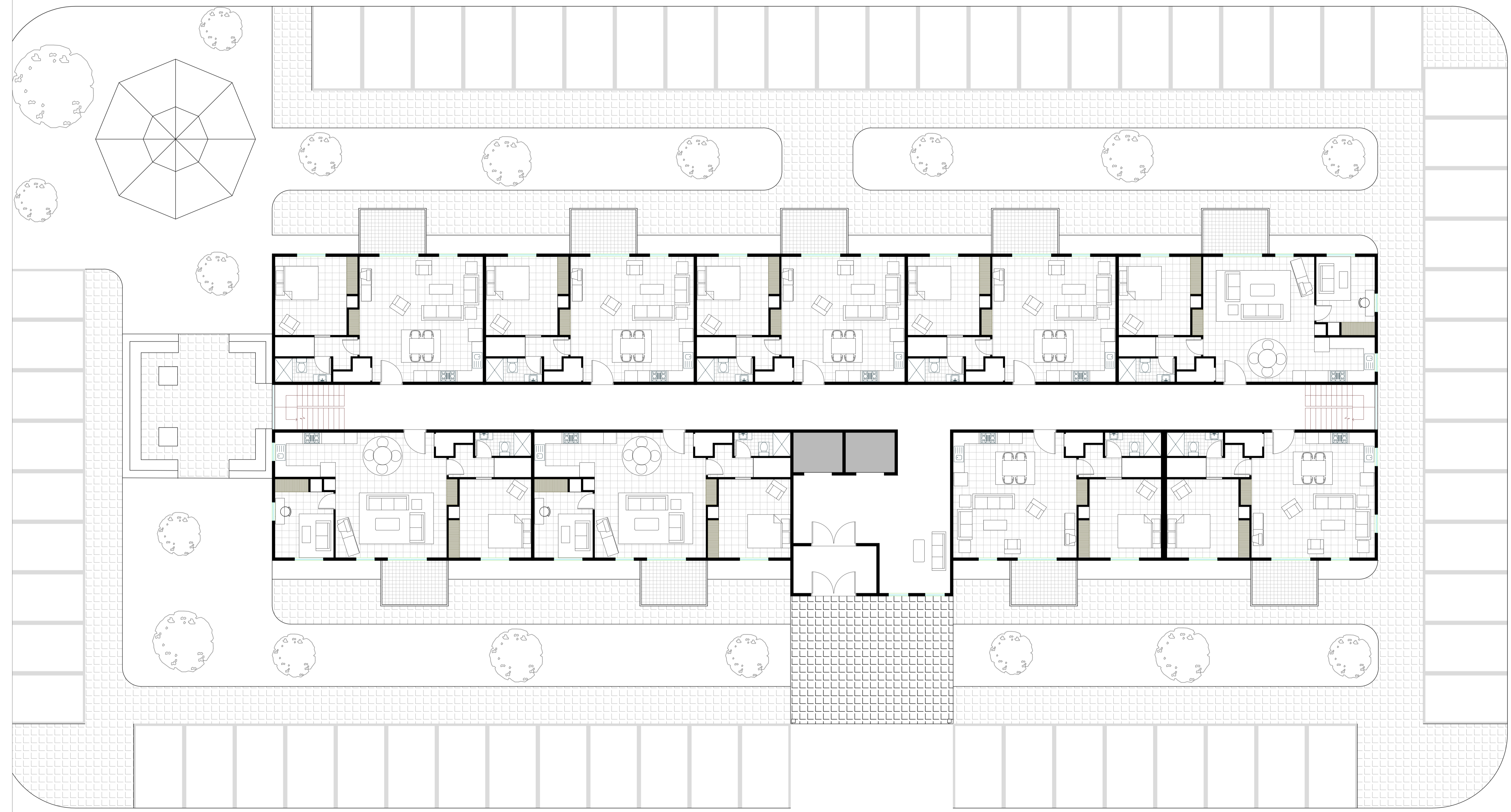
1ST FLOOR
