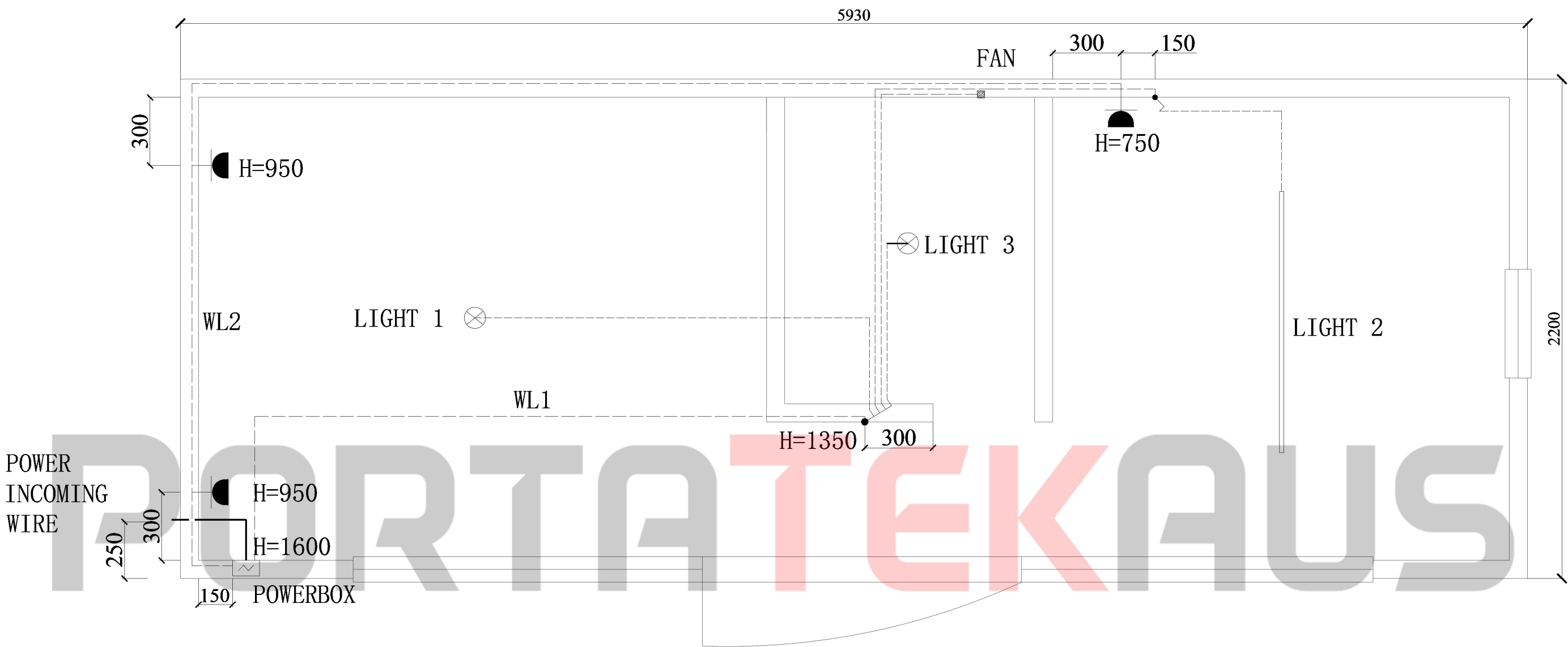
Electrical and Lighting
