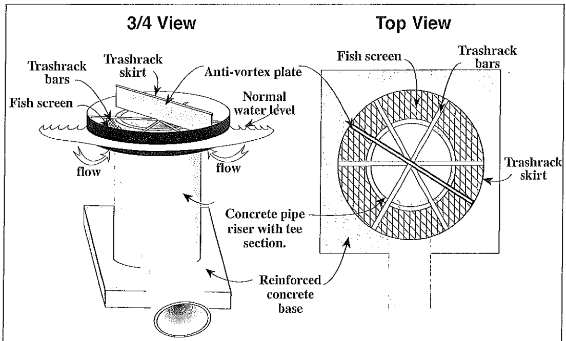
Trash Rack Design With Fish Protector Screen
