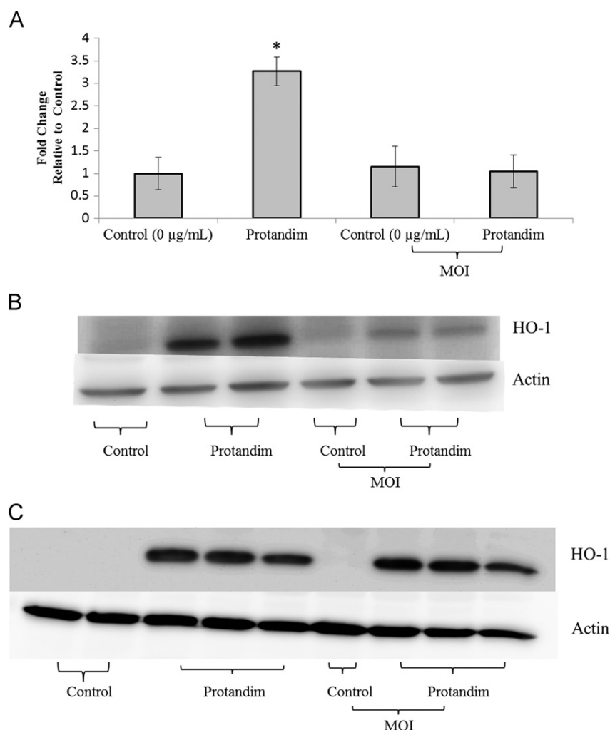
Fig. 4. Lentiviral shRNA silencing of Nrf2 abolished Protandim-induced upregulation of Nrf2 and phase II enzymes. (A) Low-density (~50% confluence) HL-1 cardiomyocytes were transduced with an MOI of 1, followed by an 8 h 100 µg/ml Protandim treatment. (B) Silencing of Nrf2 abolished phytochemically induced upregulation of HO-1 protein expression. After transduction of shRNA, HL-1 cells were treated for 12 h with 100 µg/ml Protandim and HO-1 was verified by Western blotting, with actin as a loading control. (C) HO-1 induction with phytochemical treatment was maintained with control shRNA sequence. * p < 0.05 compared to all other conditions.
