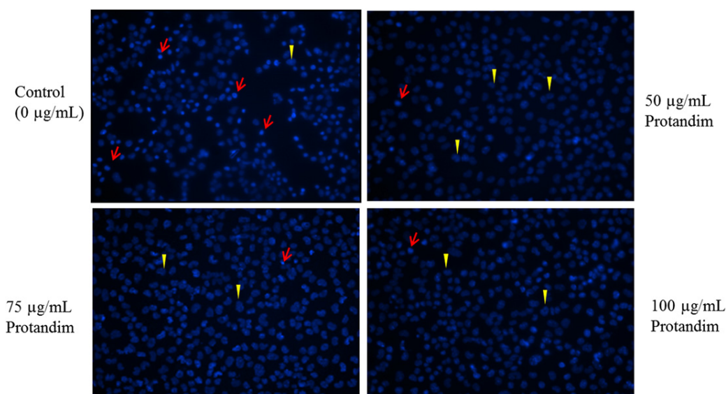
Fig. 3. Pretreatment with 50, 75, and 100 \mu\text{g/ml} Protandim protected cardiomyocytes against oxidant-induced death. Phytochemical treatment was administered for 12 h before \text{H}_2\text{O}_2 insult, and apoptosis was assessed by nuclear condensation. Red arrows identify condensed nuclei that have undergone apoptosis, and yellow triangles identify healthy nuclei that were resistant to the oxidant stress.
