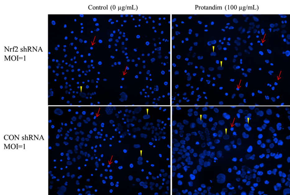
Fig. 5. Lentiviral knockdown of Nrf2 abolished protection against oxidant stress by Protandim treatment. Transduced cells were treated with 100 µg/ml Protandim or control (0 µg/ml) for 12 h, followed by a 4 h 1.25 mM H 2 O 2 insult. Apoptotic nuclei were identified by nuclear DAPI condensation and are identified by red arrows, and healthy nuclei are identified with yellow triangles. Protection remained when control shRNA was transduced.
