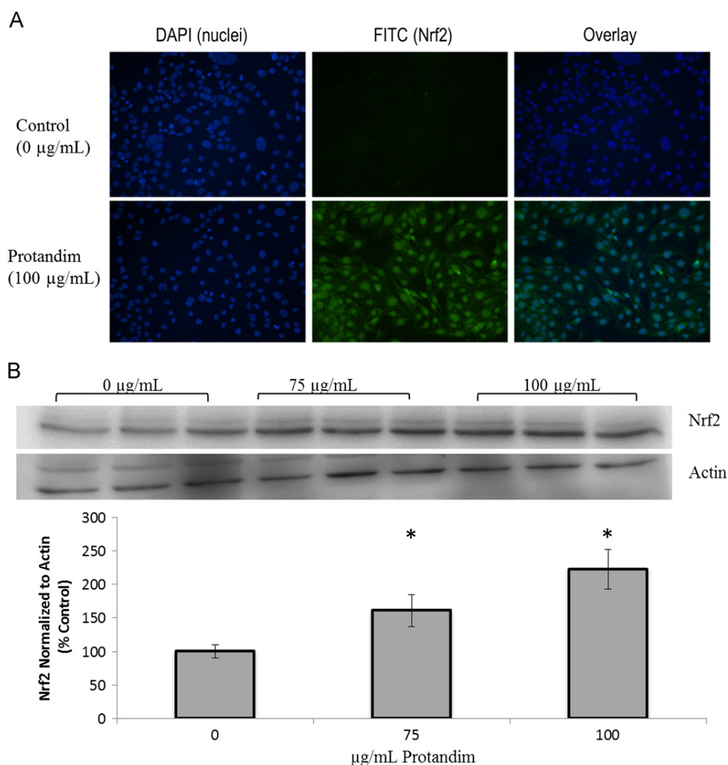
Fig. 2. Phytochemical treatment activated Nrf2. (A) HL-1 cells were treated with Protandim for 1 h and incubated with anti-Nrf2 antibody to assess Nrf2 nuclear accumulation. DAPI identifies myonuclei, and FITC identifies Nrf2. (B) Long-term treatment (48 h) with Protandim upregulated the expression of Nrf2. HL-1 cardiomyocytes were treated with 0, 75, and 100 \mu g/ml Protandim, and Nrf2 protein in the whole-cell lysate was normalized to actin. * p < 0.05 compared to control (0 \mu g/ml). n = 9 for each condition.
