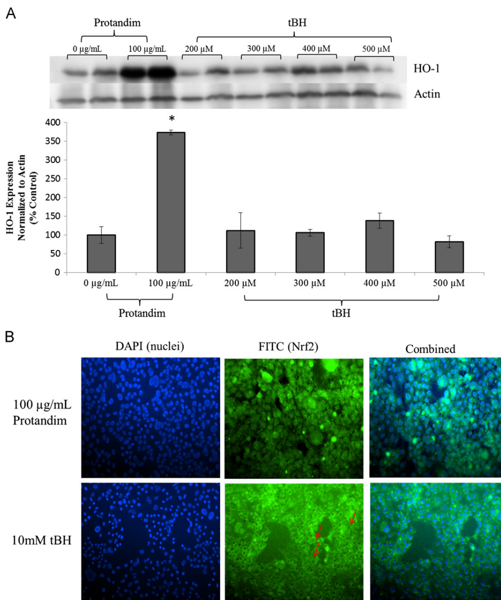
Fig. 6. Upregulation of phase II enzymes and activation of Nrf2 by Protandim treatment was more robust than by mild oxidant stress. (A) HL-1 cardiomyocytes were treated for 12 h with 100 \mu\text{g/mL} Protandim or for 12 h with varying concentrations of tBH. HO-1 expression was normalized to actin and expressed as a percentage of the 0 \mu\text{g/mL} control; n=2 in each condition. (B) Oxidant stress did not activate Nrf2 and induce nuclear accumulation. Whereas 2 h treatment with Protandim resulted in nuclear accumulation of Nrf2, 2 h of 10 mM tBH insult did not induce nuclear accumulation, but tended to promote nuclear exclusion and cytosolic enrichment. Arrows identify nuclear exclusion.
