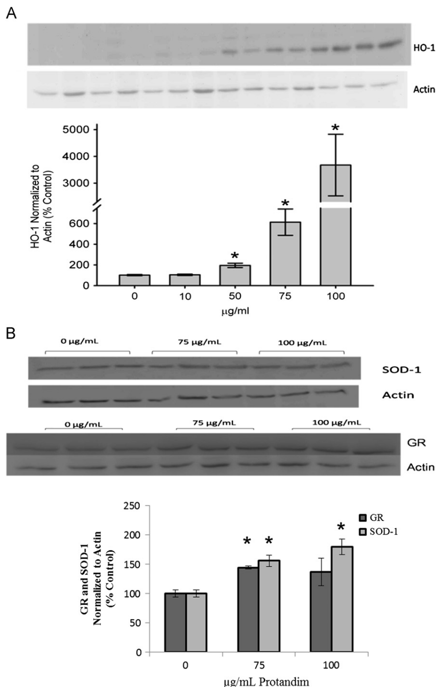
Fig. 1. Treatment with phytochemicals upregulated the expression of phase II enzymes in a concentration-dependent manner. (A) 12 h of Protandim treatment significantly upregulated HO-1 expression at 50, 75, and 100 µg/ml, with greatest induction of 300-fold over control (0 µg/ml) observed with 100 µg/ml. (B) 12 h of phytochemical treatment significantly upregulated expression of SOD-1 and GR. * p < 0.05 compared to control (0 µg/ml). n=9 for each condition.
