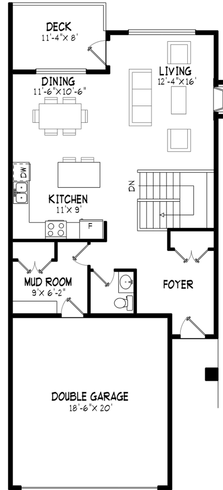
MAIN FLOOR FINISHED FLOOR AREA = 814 SQ.FT. GARAGE AREA = 398 SQ.FT.
