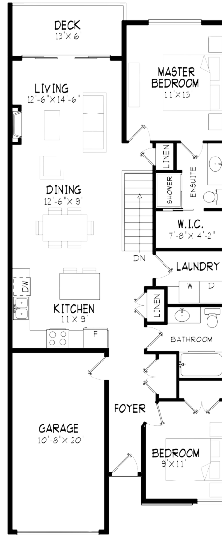
MAIN FLOOR FINISHED FLOOR AREA = 1110 SQ.FT. GARAGE AREA = 229 SQ.FT.
