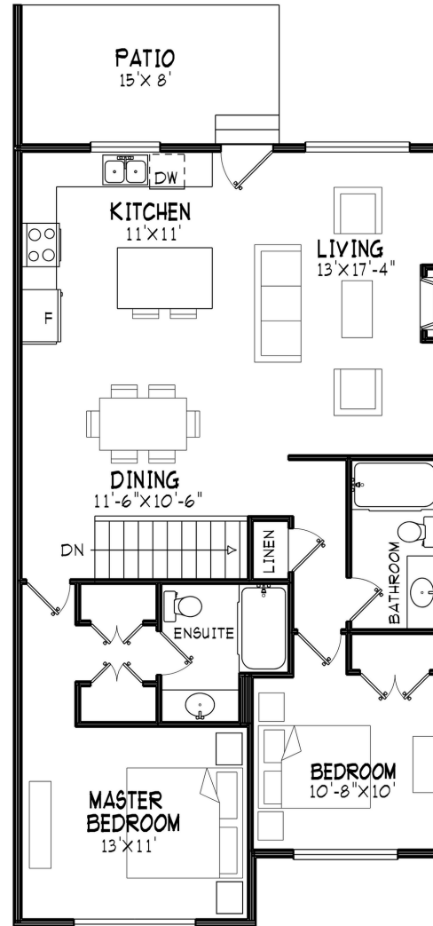
MAIN FLOOR FINISHED FLOOR AREA = 1060 SQ.FT.
