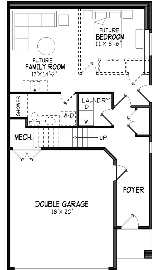
LOWER FLOOR FLOOR AREA = 728 SQ.FT. GARAGE AREA = 382 SQ.FT.
