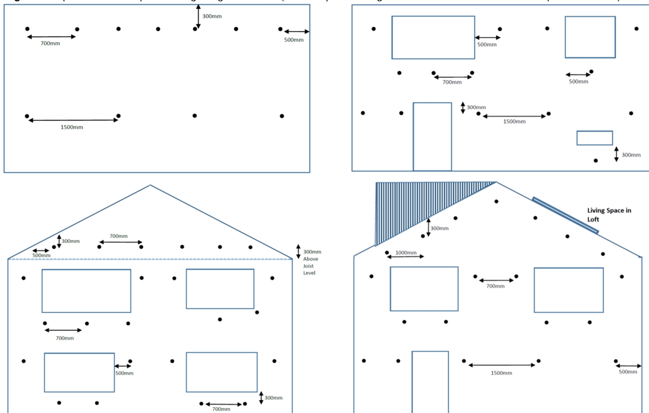
Diagram 1 - Optional full fill drill pattern using straight cut nozzle (main drill pattern using Climabead nozzle is detailed in the Operation Manual)
