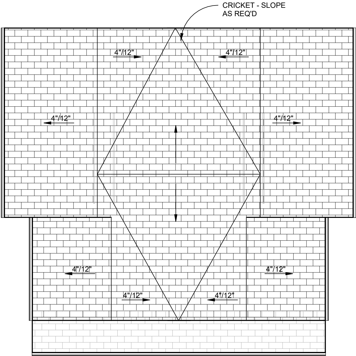
2 ROOF PLAN 1/8" = 1'-0"
