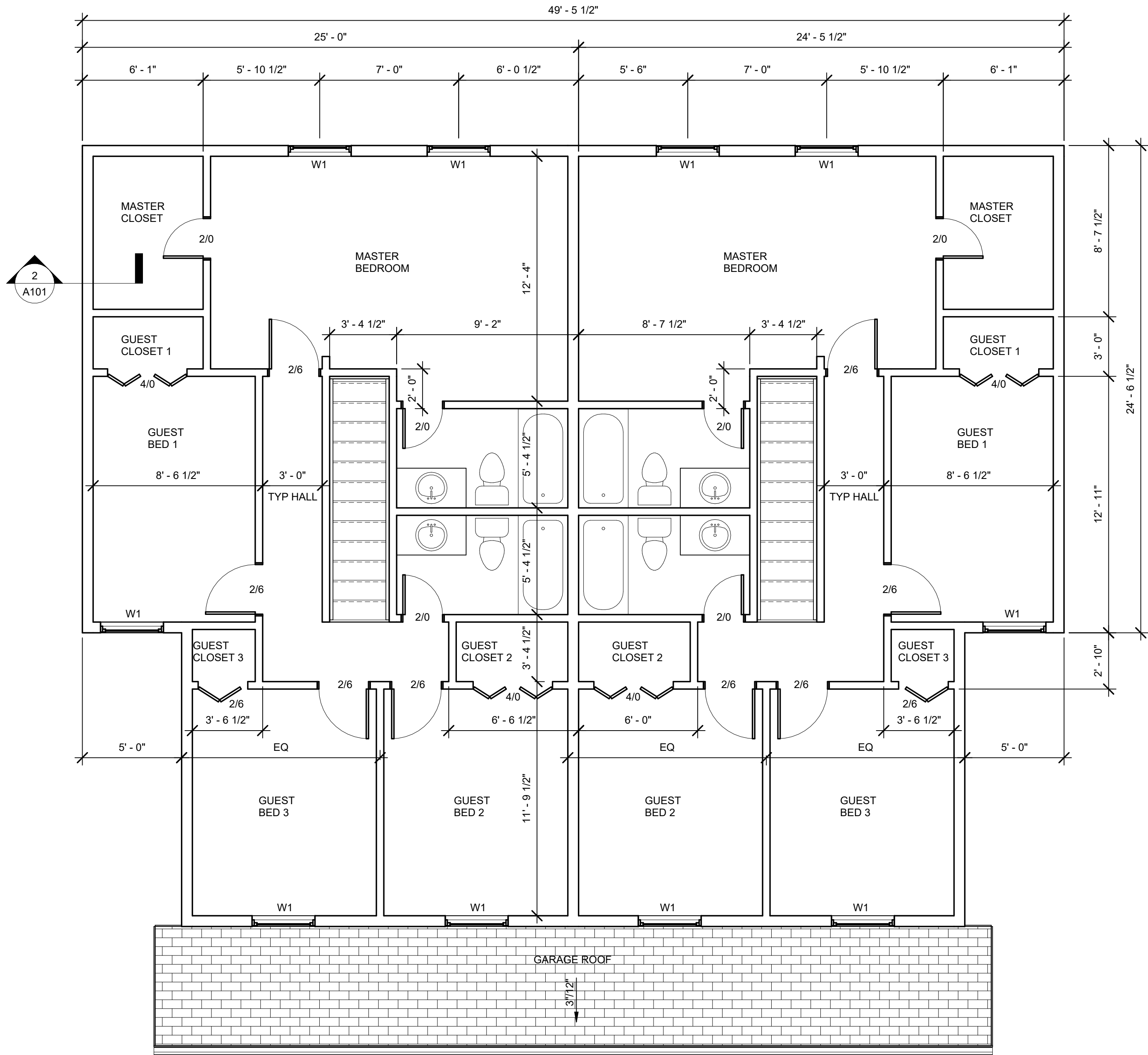
3 SECOND FLOOR PLAN 1/4" = 1'-0"
