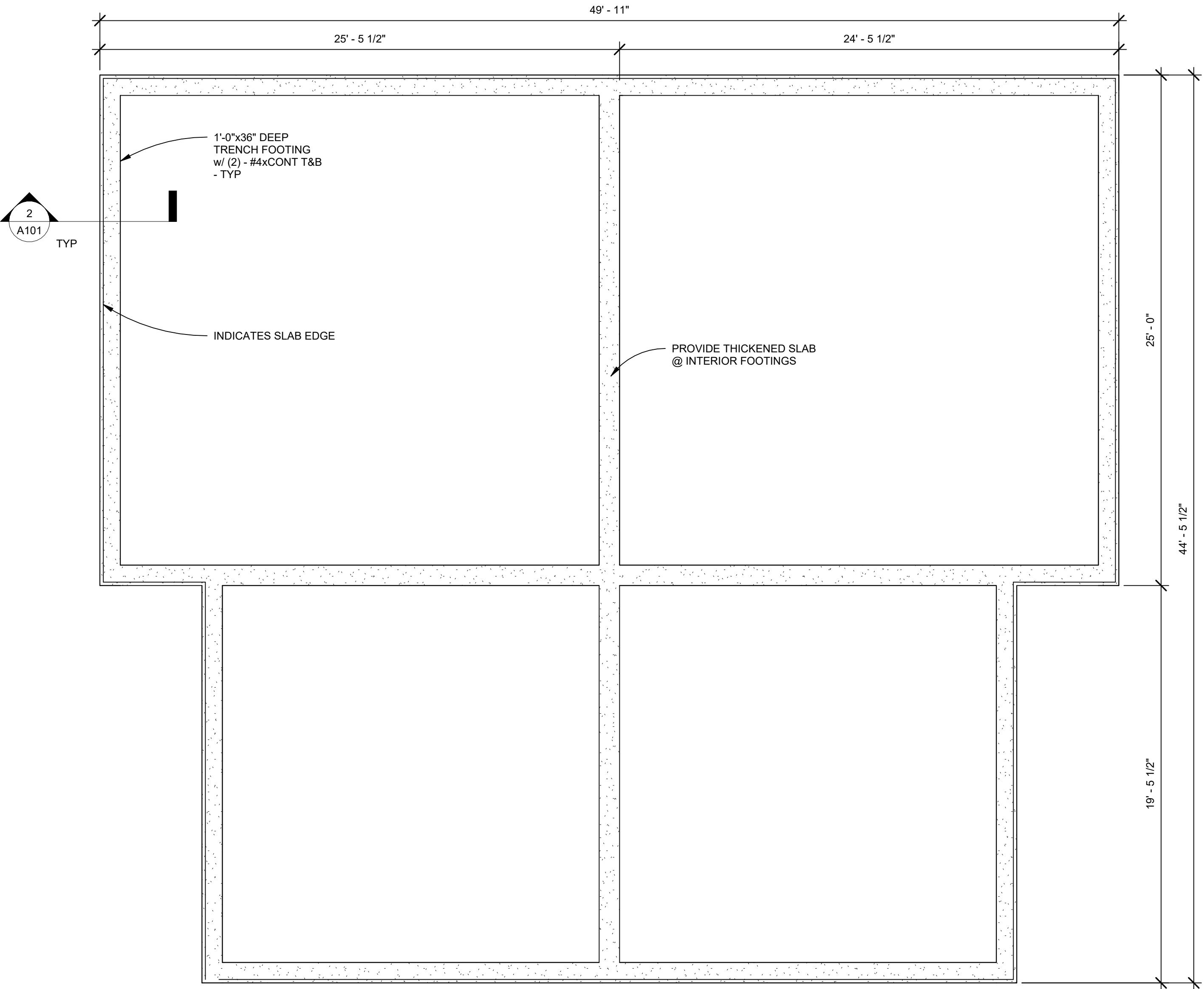
① FOUNDATION PLAN 1/4" = 1'-0"
