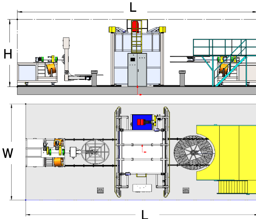
Shuttle machine install layout
