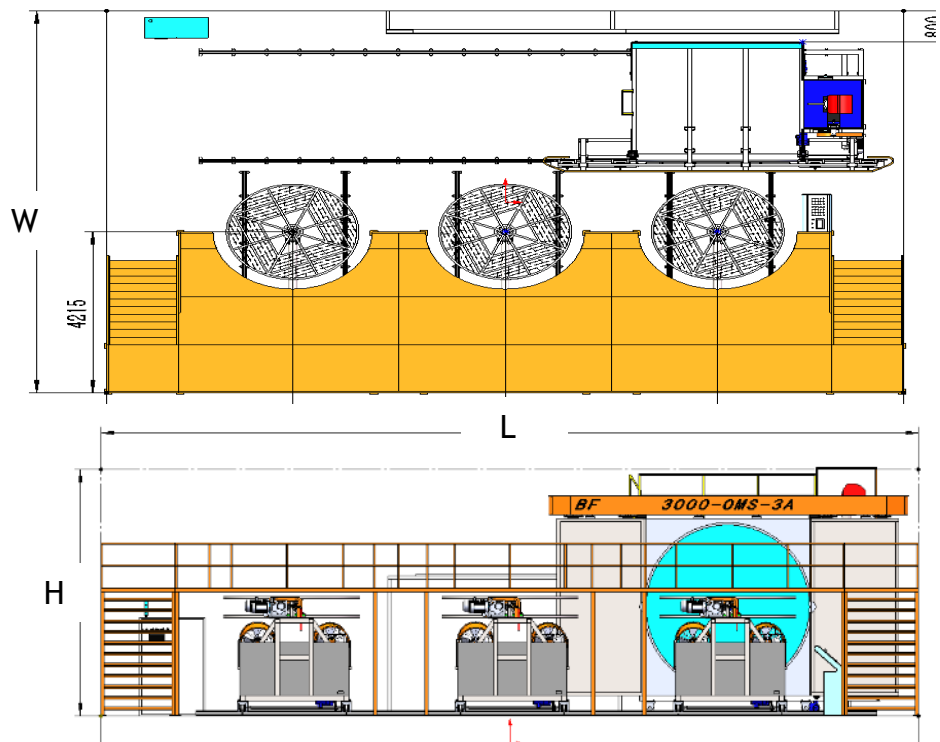
OMS machine install layout
