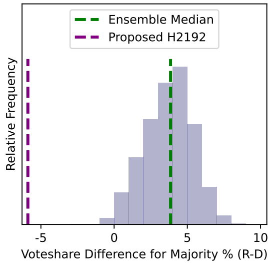
"Mean-Median" Score
