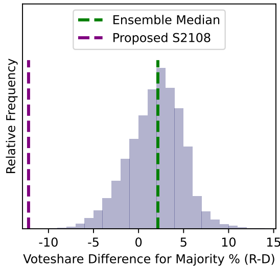
"Mean-Median" Score
