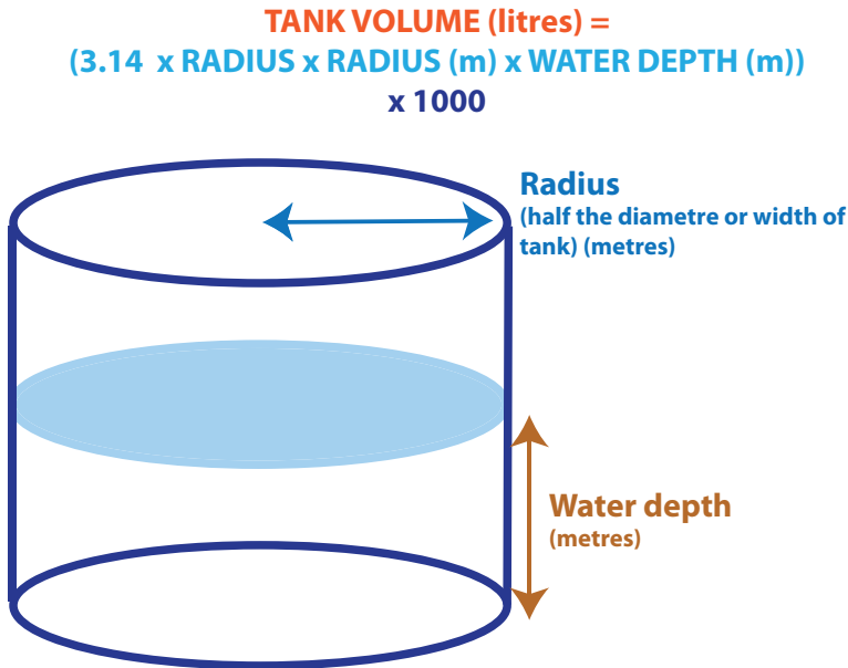
Figure 5: Calculating tank volume
