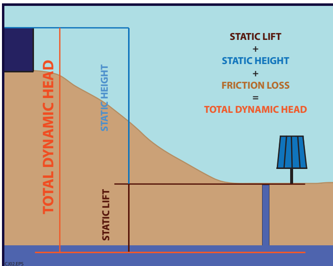
Figure 2: Total dynamic head
