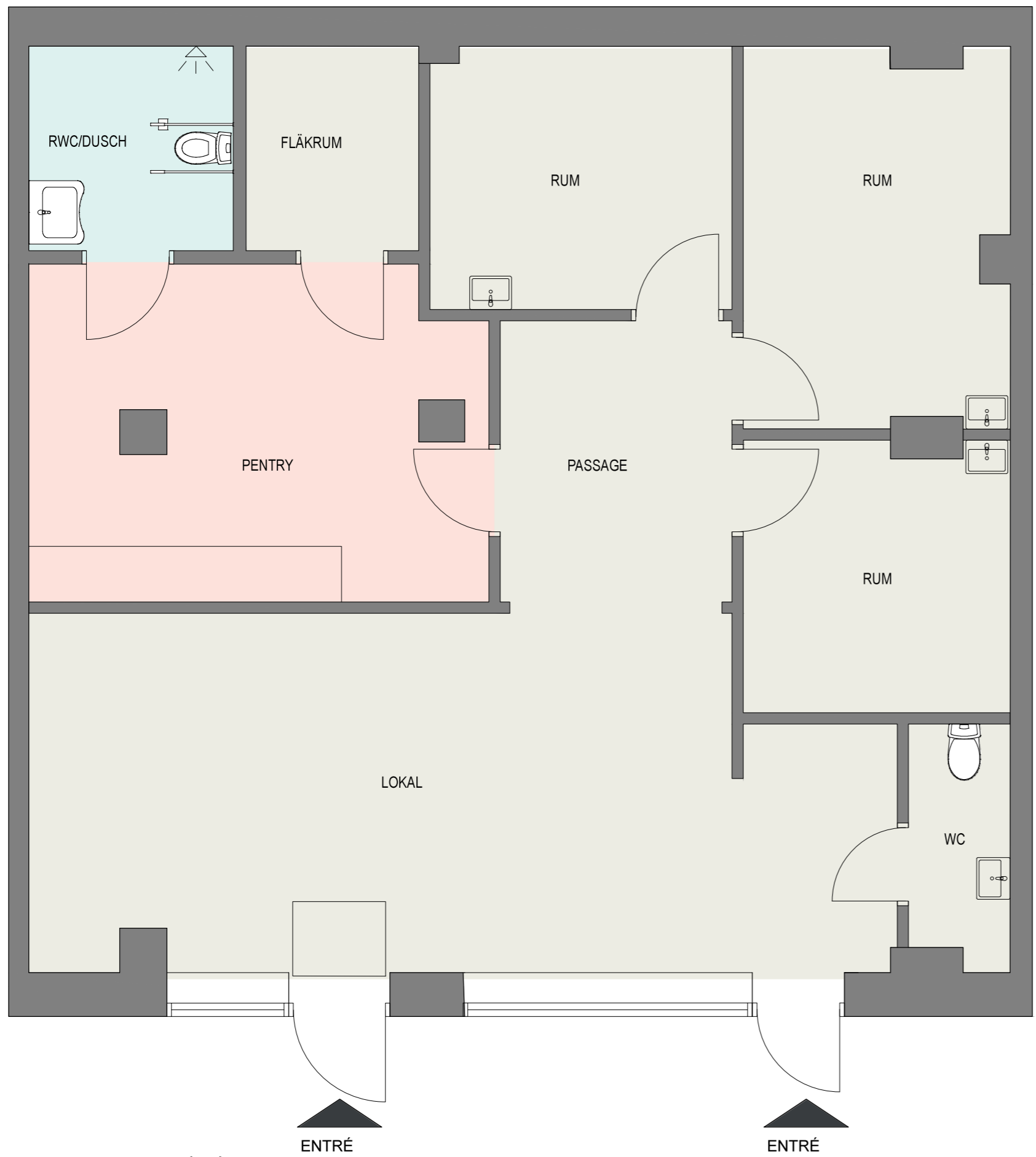
PLAN SKALA 1:50 (A3)
