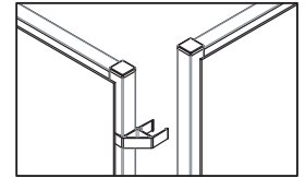
Two Panels 90° Use one pair of Corner QuickConnectors
