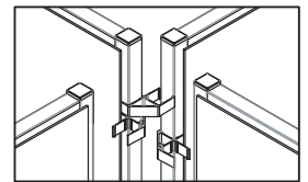
Four Panels Use three pair of Corner QuickConnectors
