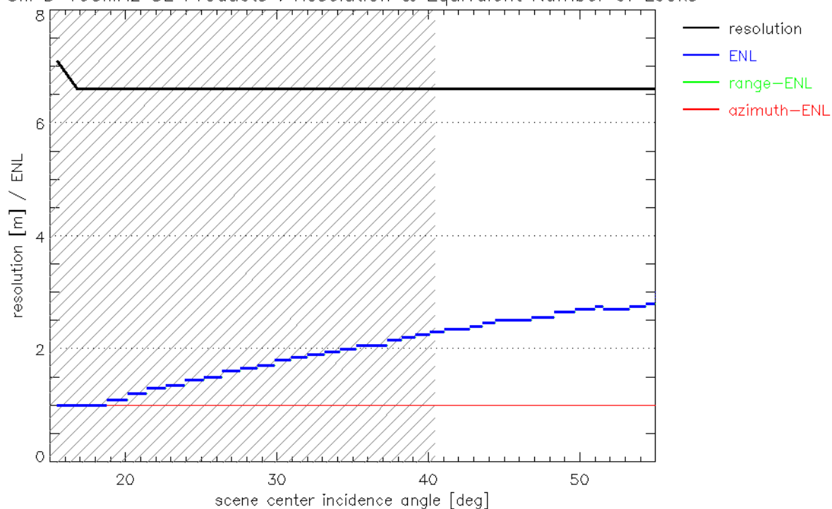
SM D 100MHz SE Products : Resolution & Equivalent Number of Looks
