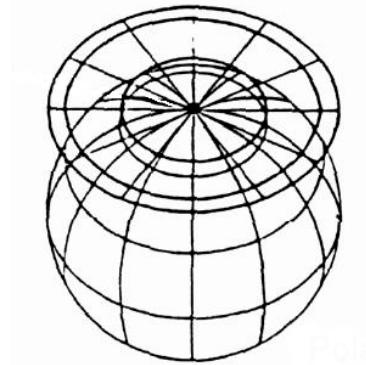
Fig. 3-16: Polar Stereographic Projection. Figure taken from [RD 3].
