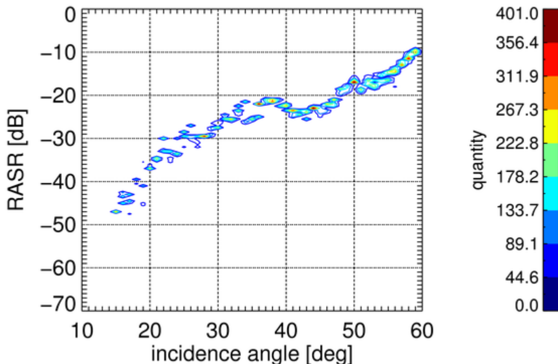
Figure 10 Simulated RASR of the worst target over range for more than 20000 statistical acquisitions. The contour lines of the two dimensional histogram are given, highlighting the dominant regions of predicted RASR.
