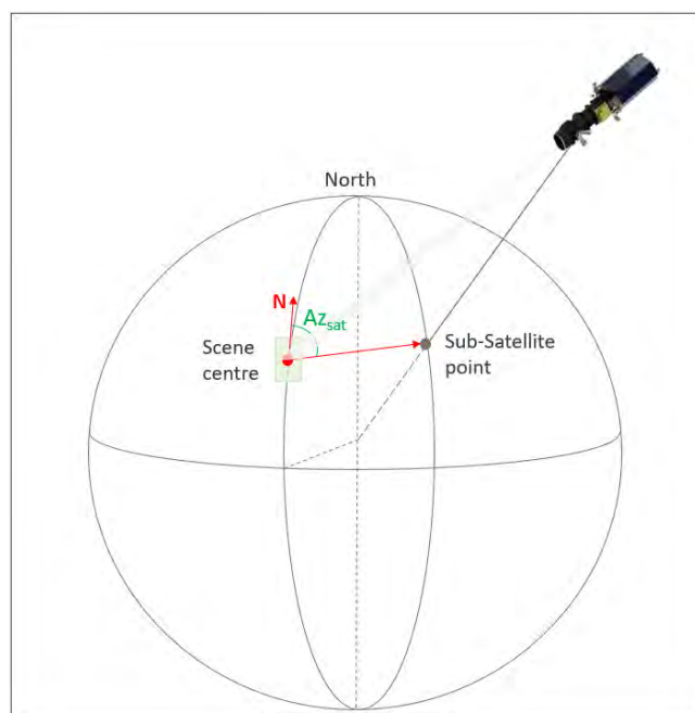
Figure A-3: Definition of the sensor azimuth angle
