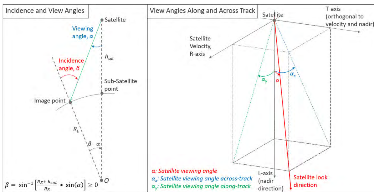
Figure A-2: Definitions of incidence and view angles in general (left); and projected along and across track (right)
