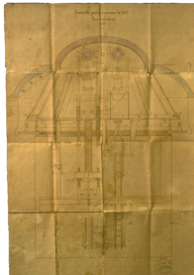
Lot. 8554 ..... Starting Price: 50 € "Tourelle pour 2 canons de 15 c/m. Coupe transversale, Ech. 1/10, Societe Norddenfelt, 1-10-1894". Μεγάλο σχέδιο κανονιών του 1894. Very large drawing of two canons, 1894. Size: 70 x 100 cm.
