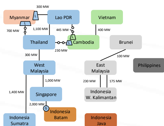
Figure 5.4.1-2 Regional Interconnections Evolution
