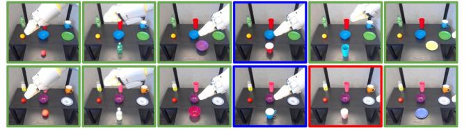
Fig. 8. The robot experiment of pointing to the best match of a query object (placed in front of the robot on the small table). The closest match is selected from two sets of target objects, placed on the table behind the query object. The first and the second row correspond to the experiment for the first and second target set. Images with green frame indicate cases where both the ‘class’ and ‘container’ attributes are matched correctly. Blue frames show where only the ‘container’ attribute is matched correctly and red frames indicate neither attribute is matched.
