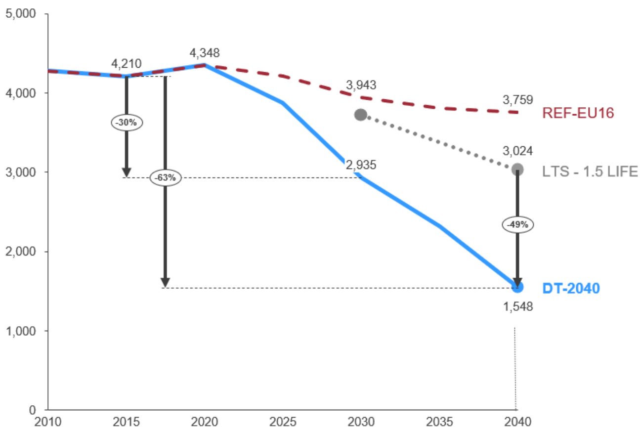
Figure 7: Yearly energy consumption: Comparison between baseline scenario (EU-REF16), EU LTS 16 and DT-2040 scenario (international shipping excluded) 14 (TWh)
