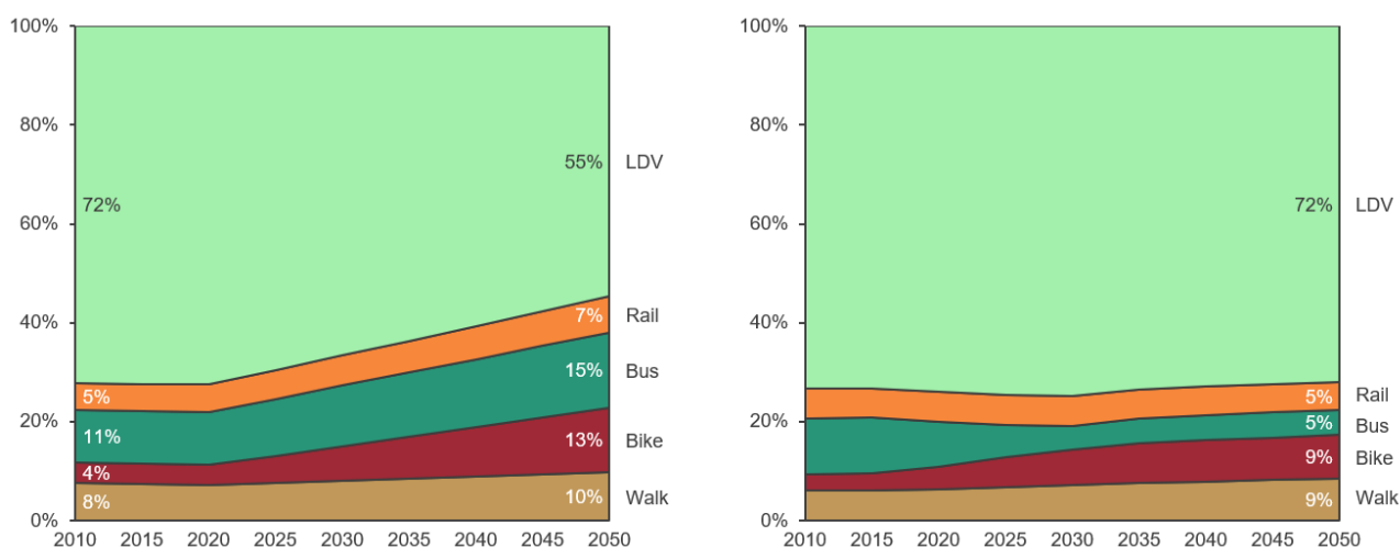
Modal share evolution in DT-2040 scenario for passenger transport (% of passenger kilometres) Modal share evolution in REF-EU16 scenario for passenger transport (% of passenger kilometres)
