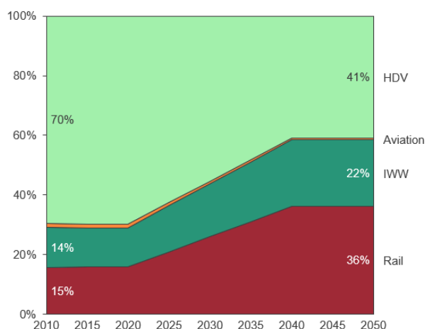
Modal share evolution in DT-2040 scenario for freight transport (% of tonne-kilometres)
