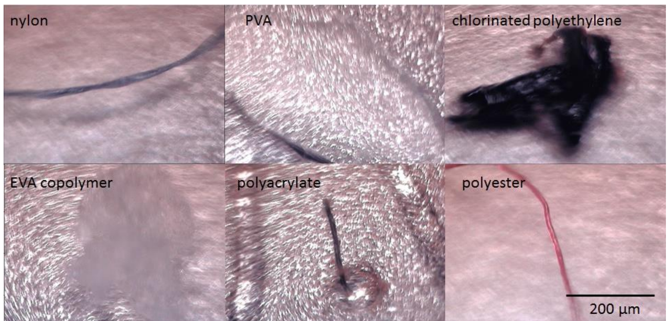
Figure 2: some examples of the microplastic fibres and fragments found in surface water samples from the Vltava-Labe river system, and their identities as determined by FT-IR microscopy.
