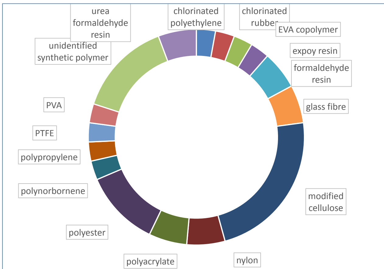
Figure 4: the diversity of synthetic fibres and fragments, including microplastics, found across all samples combined, with an indication of their relative abundances.
