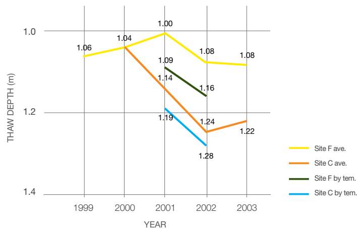
Figure 4 Permafrost loss as a result of clearcut logging
