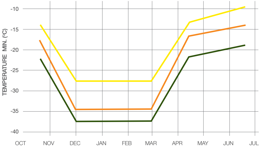
Figure 1 Mountain pine beetle cold-mortality thresholds
