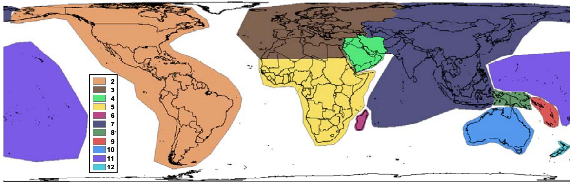
Figure S4: Bird Distribution Data Sources. A map illustrating the core references used for geographic sub-regions. Select additional sources such as island species lists were used.
