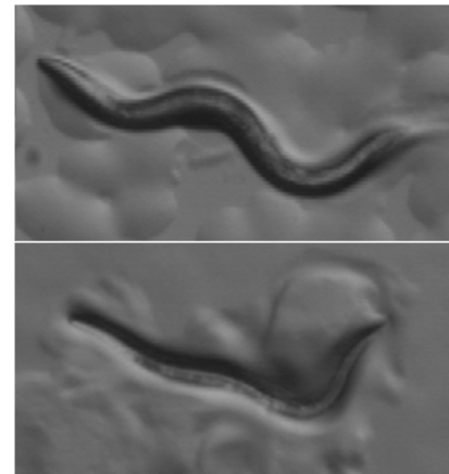
A five-subunit acetylcholine channel coordinates muscle contraction and relaxation by regulating motor neuron excitability in C. elegans , allowing the worm to move in a sinusoidal manner (top panel). A mutation in the pore-lining domain of the ACR-2 subunit causes muscle hyper-contraction, due to imbalanced inputs from the motor neurons (bottom panel). (The worm’s head is to the left.) (Image Credit: Tamara M. Stawicki and Yishi Jin). doi:10.1371/journal.pbio.1000268.g001
