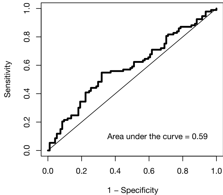
ROC curve for test set
