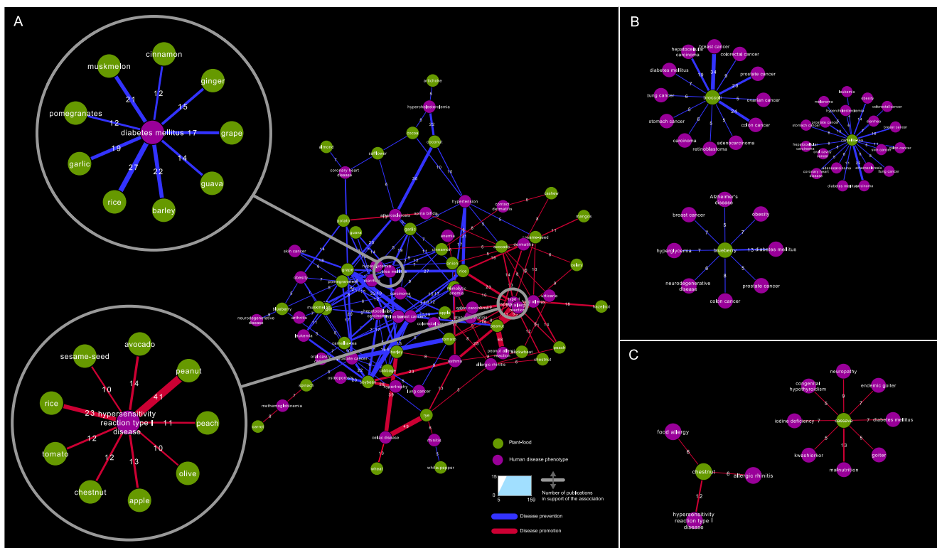
Figure 3. Food – disease association network. a) Disease phenotypes associated with common vegetables, fruits and plants of our diet. Foods are shown as green nodes and human disease phenotypes as purple nodes. Disease prevention/amelioration is depicted as a blue edge and disease promotion as a red edge. The size of the edge indicates the number of publications in support of the association. An edge is drawn between a food node and a disease node when there are at least five publications in support of this association. When a disease node has more than five edges, only the five strongest (with the most publication support) are shown on the network for the sake of clarity. Top left: zoom in the network formed between diabetes mellitus and foods that prevent/ameliorate the disease. Bottom left: zoom in the network formed between Type 1 hypersensitivity and foods that promote it. b) Examples of a vegetable (broccoli), a fruit (blueberry) and a plant-based beverage (camellia-tea) that are only positively associated with disease phenotypes. c) Two examples of foods that are only negatively associated with disease phenotypes. doi:10.1371/journal.pcbi.1003432.g003
