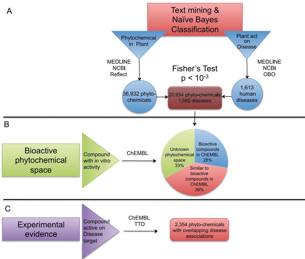
Figure 4. Association of phytochemicals to human disease phenotypes. The flow diagram illustrates the approach we followed for associating phytochemicals to human disease phenotypes. a) In the phytochemical - food and food - disease relations that we extracted by text mining, there are 7,077 plants with both phytochemical and human disease annotation. We used Fisher's exact test to identify statistically significant correlations between phytochemical and human disease phenotypes. At a 5% false discovery rate we identified 20,654 phytochemicals associated to 1,592 human disease phenotypes. b) 5,709 of the text-mined phytochemicals have been tested experimentally on a biological target and the activity data have been deposited in ChEMBL. For the remaining two thirds of the compounds, 8,113 phytochemicals are structurally similar to compounds with known protein targets (estimated with a Tanimoto coefficient >0.85 ), indicating similar bioactivity. The rest of the compounds, 6,832 phytochemicals, are not similar to any known bioactive compound and belong to a hitherto unexplored phytochemical space. c) We used the Therapeutic Targets Database to annotate the protein targets from ChEMBL to diseases. From the 5,709 phytochemicals that are included in ChEMBL, 2,354 are active against a biological target that is relevant for the same disease as the one we have predicted. doi:10.1371/journal.pcbi.1003432.g004
